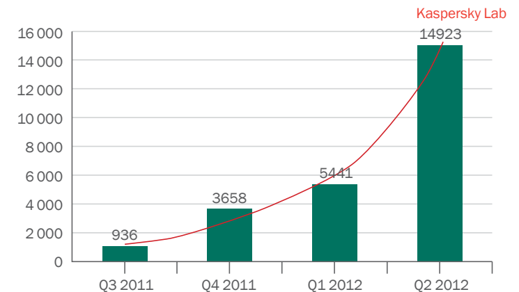
Fig 4: The number of malware modifications targeting Android OS
